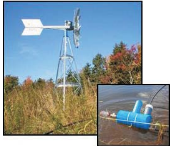
Picture 5: A 12-foot windmill driving a water pump with compressed air
